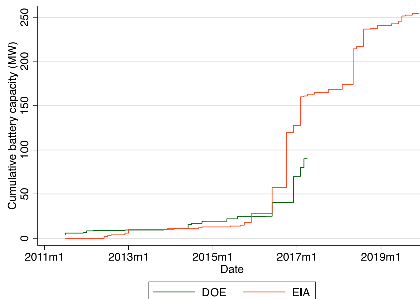
Fig. A.9. Installed battery capacity CAISO. Notes: Cumulative installed battery capacity in CAISO.
