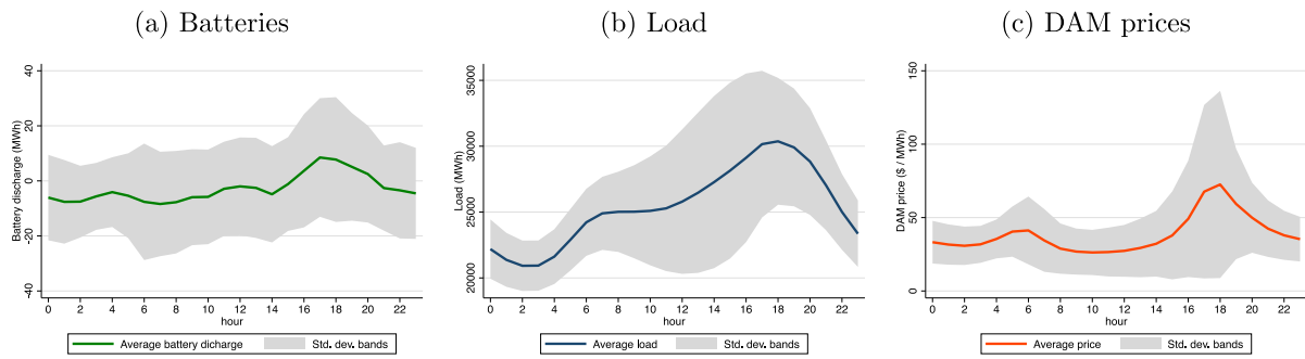
Fig. 1. Batteries output, load, and prices from the CAISO.
